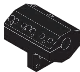
SPLIT BORING BAR HOLDER ..... pg 62
