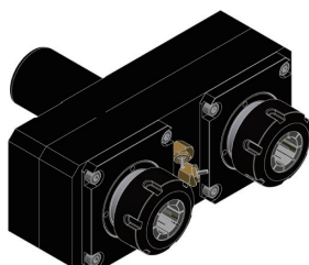
DOUBLE OFFSET STRAIGHT DRILL - MILLING LIVE TOOL ..... pg 43
